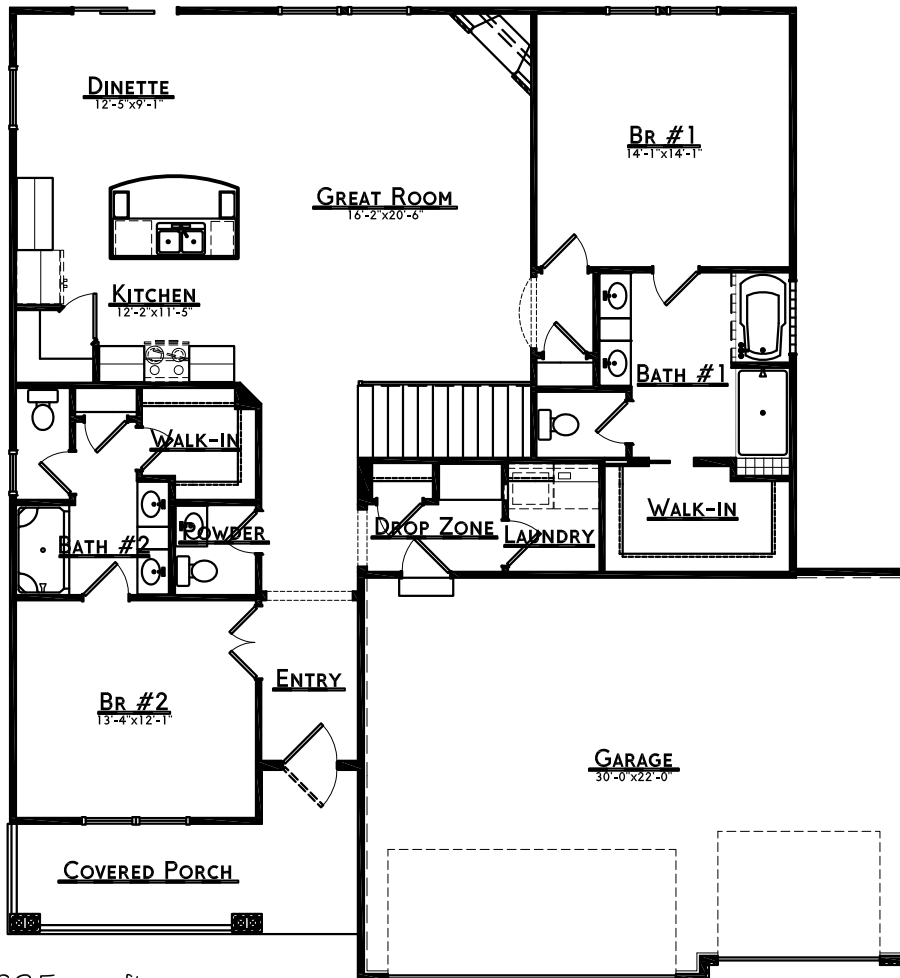
MAIN LEVEL - 1635 sq ft
