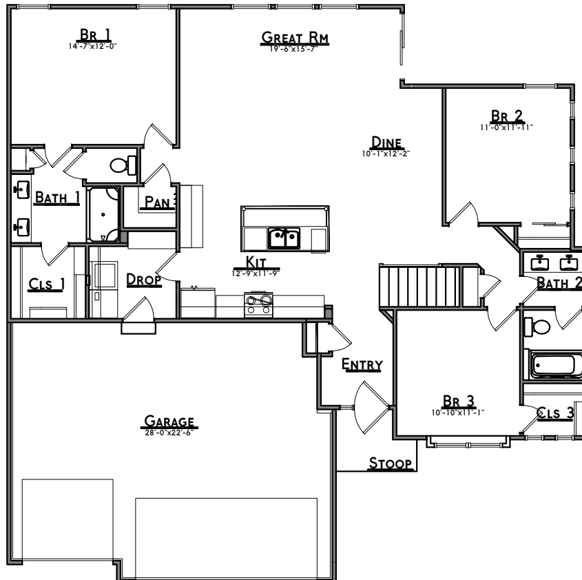
MAIN LEVEL - 1538 sq ft
