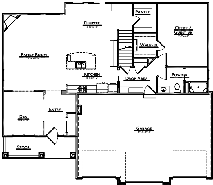
MAIN LEVEL - 1542 sq ft
