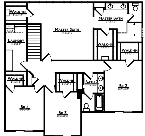
UPPER LEVEL - 1419 sq ft
