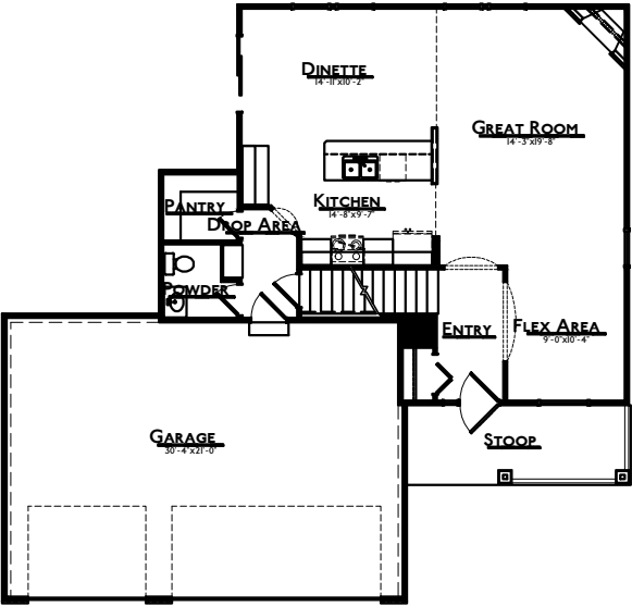
MAIN LEVEL - 912 sq ft
