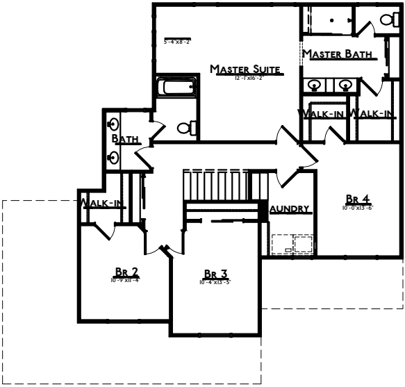
UPPER LEVEL - 1240 sq ft
