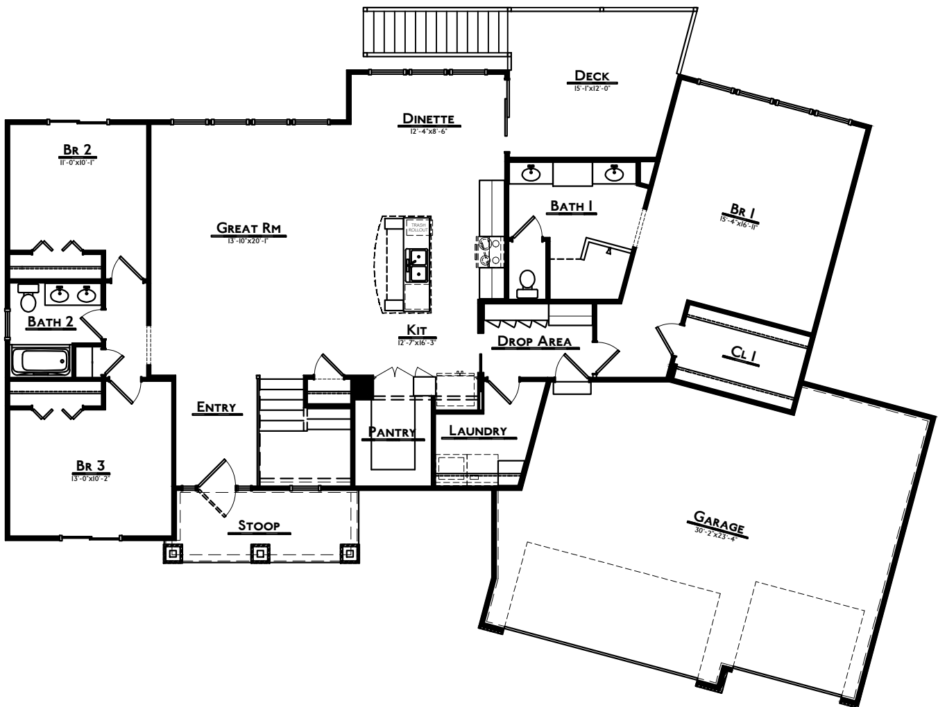
MAIN LEVEL - 1879 sq ft
