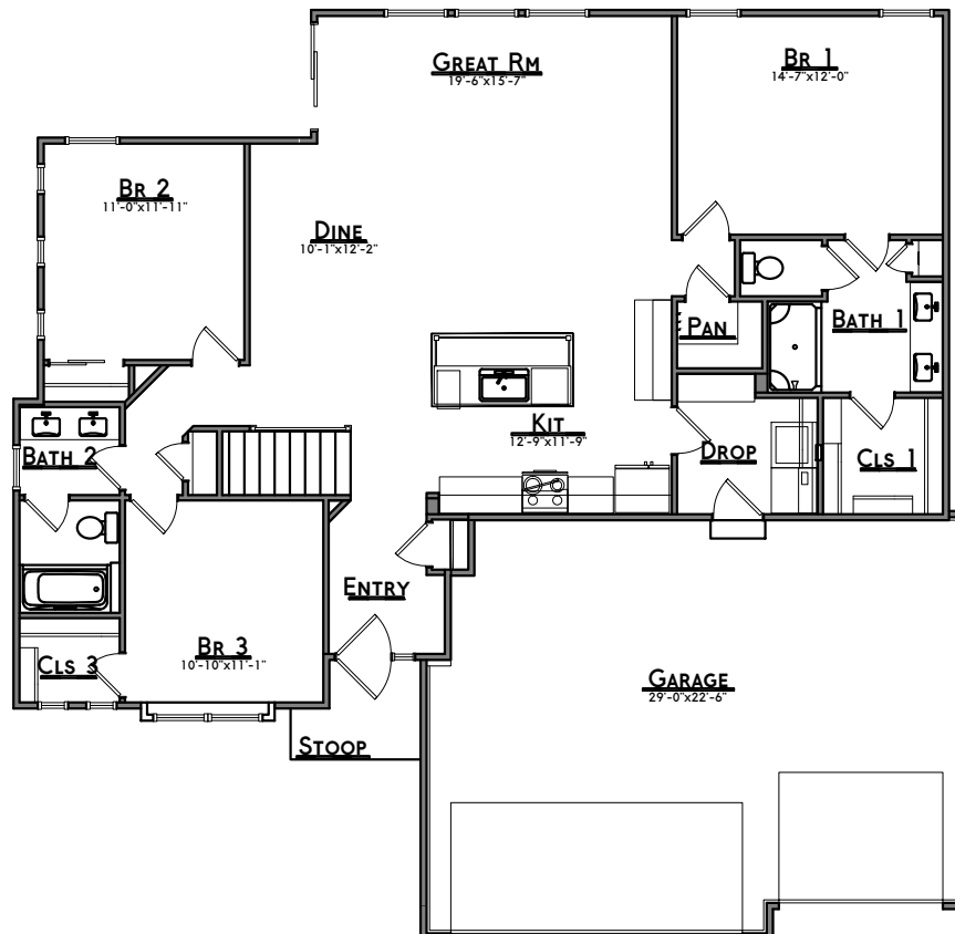
MAIN LEVEL - 1538 sq ft
